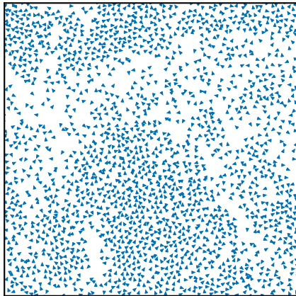
Disordered \eta = 0.3, \langle \varphi \rangle = 0.25
