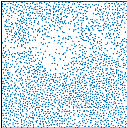
Near-critical \eta = 0.1, \langle \varphi \rangle = 0.63
