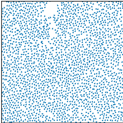
Ordered \eta = 0.02, \langle \varphi \rangle = 0.83
