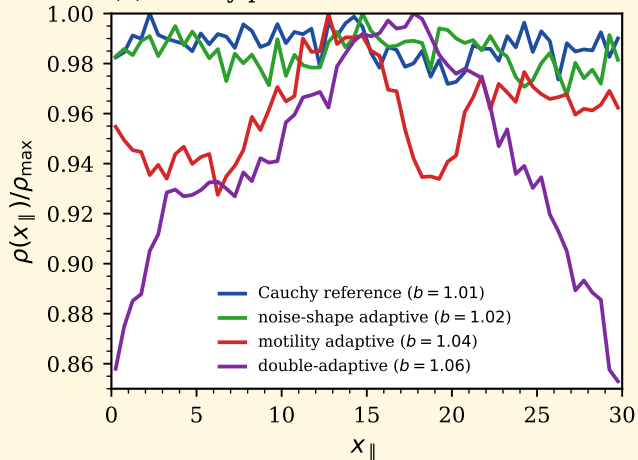
(a) density profile
