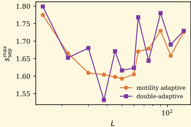
(a) s_{\text{sep}}^{\text{max}}(L)
