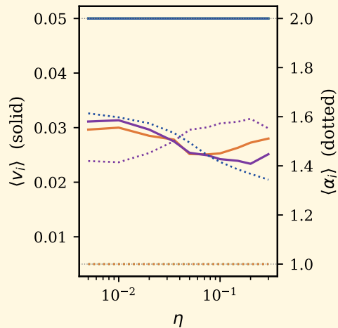
(f) \langle v_i \rangle , \langle \alpha_i \rangle vs \eta
