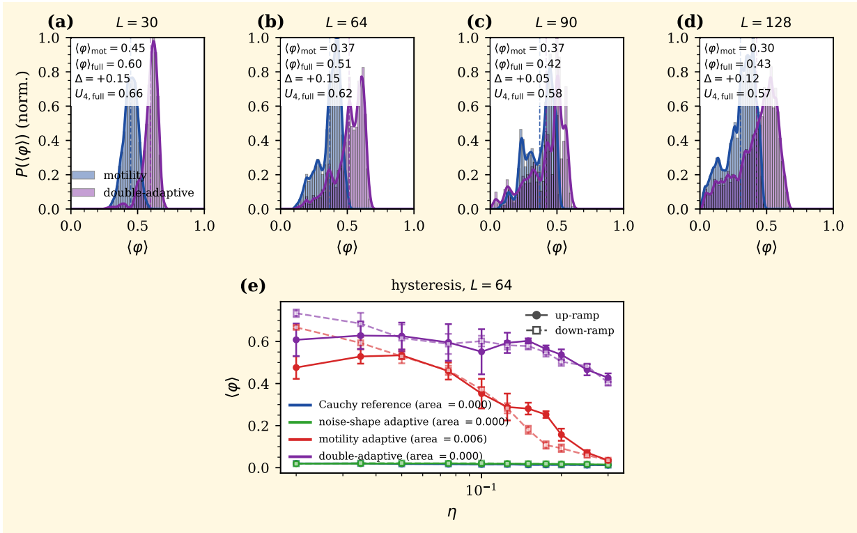
Figure S1. Order of the transition. (a)–(d) order-parameter distribution P(\langle\varphi\rangle) with motility-only and double-adaptive overlaid, one panel per size (a) L = 30 , (b) L = 64 , (c) L = 90 , (d) L = 128 (motility at \eta = 0.10 , double-adaptive at \eta = 0.15 ), each normalised to its own peak and sharing the vertical scale; dashed lines mark the per-mode means and each panel reports the mean gap \Delta and the full-mode Binder cumulant U_4 . (e) quasi-static \eta ramp up (filled circles, solid) and down (open squares, dashed) at L = 64 , five seeds, all four modes (hue), with the loop areas. P(\langle\varphi\rangle) stays single-peaked at every size and the hysteresis loops are negligible ( \leq 0.006 ): the deepened Binder dip is not a coexistence signature and the transition is continuous (at most very weakly first-order).
