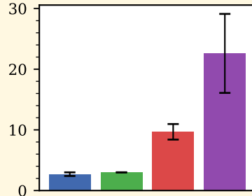
(c) mean cluster size
