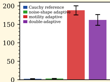
(a) cluster count
