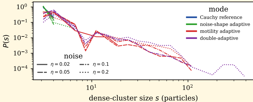
(e) cluster-size distribution
