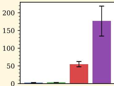
(b) max cluster size
