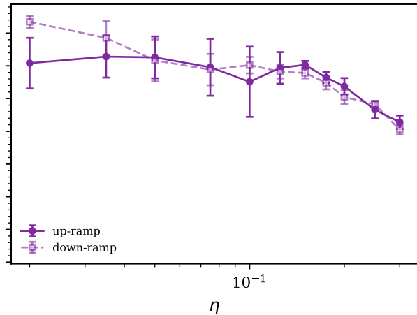
double-adaptive (area = 0.000)
