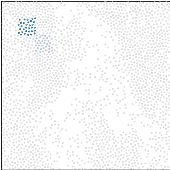
motility adaptive \eta = 0.1, \langle \phi \rangle = 0.52, n_{cl} = 2
