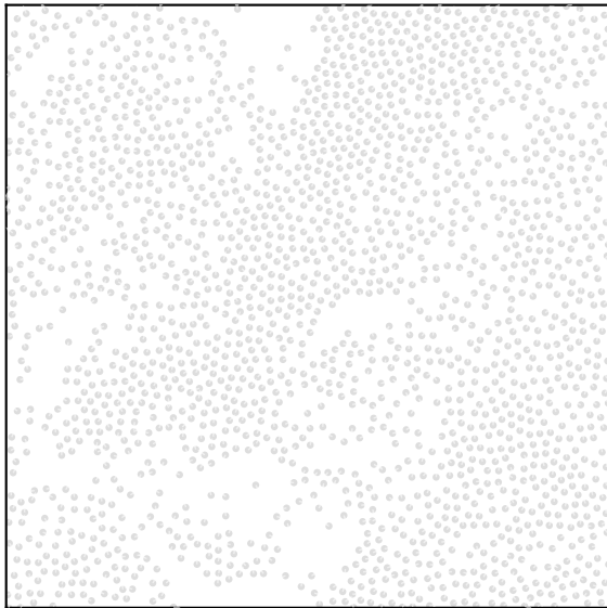
double-adaptive \eta = 0.1, \langle \phi \rangle = 0.66, n_{cl} = 0
