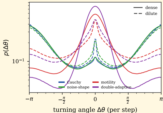
(c) turning-angle pdf
