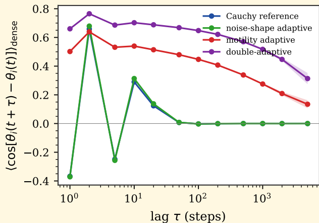
(a) dense-quartile C(\tau)
