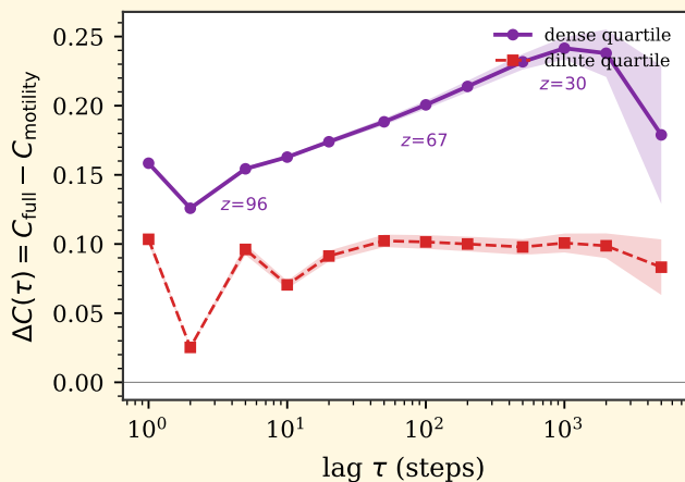
(b) full – motility gap
