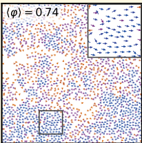
(a) ordered, \eta = 0.02
