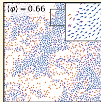
(b) near critical, \eta = 0.1
