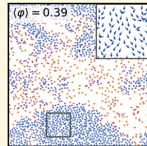
(c) disordered, \eta = 0.3
