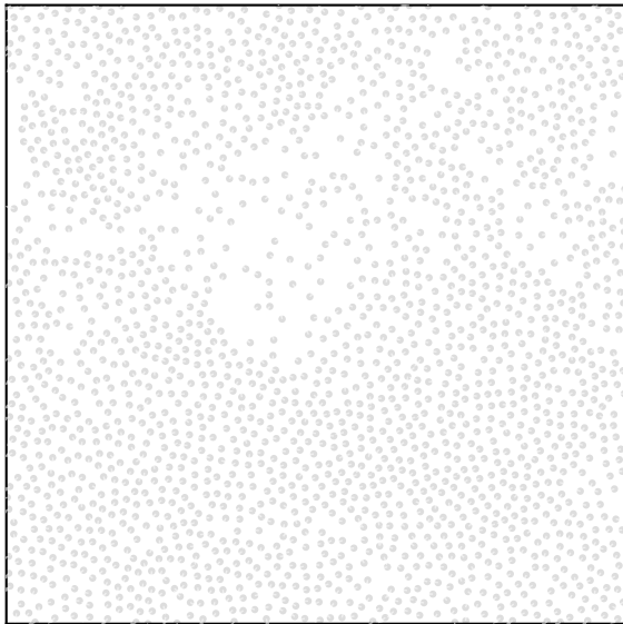
double-adaptive \eta = 0.1, \langle \varphi \rangle = 0.63, n_{cl} = 0
