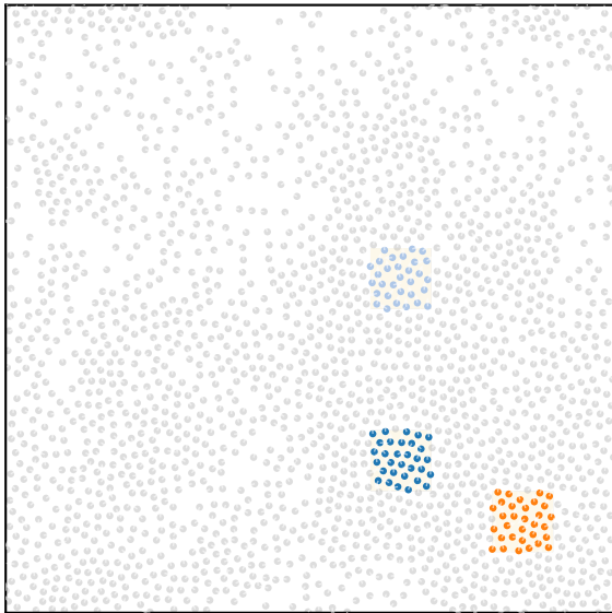
motility adaptive \eta = 0.1, \langle \varphi \rangle = 0.47, n_{cl} = 3
