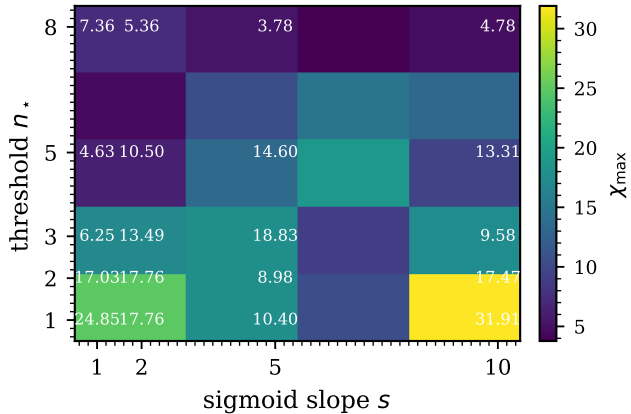
(a) \chi_{\max} (full mode, L = 30 , 5 seeds)
