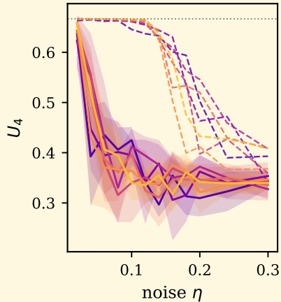
(c) Binder cumulant \alpha = 1 solid, \alpha = 2 dashed
