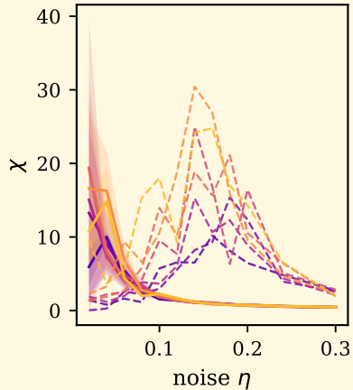
(b) susceptibility \alpha = 1 solid, \alpha = 2 dashed
