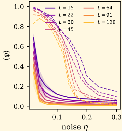
(a) order parameter \alpha = 1 solid, \alpha = 2 dashed
