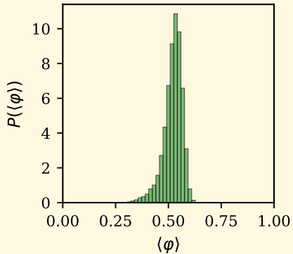
topological, \alpha = 1 , \eta = 0.20 new transition
