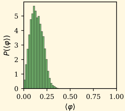
metric, \alpha = 1 , \eta = 0.05 continuous ref
