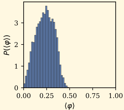
topological, \alpha = 2 , \eta = 0.50 Ginelli--Chate
