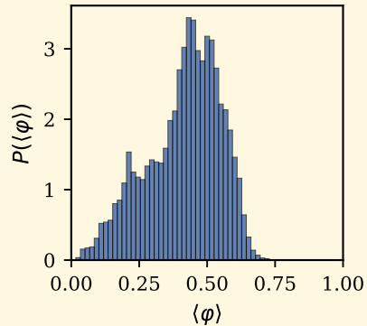
metric, \alpha = 2 , \eta = 0.15 first-order ref
