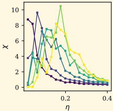
(b) susceptibility
