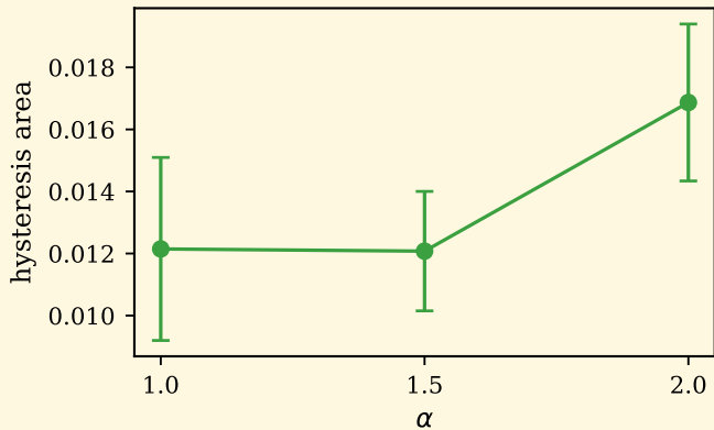
(c) spatial MSD exponent
