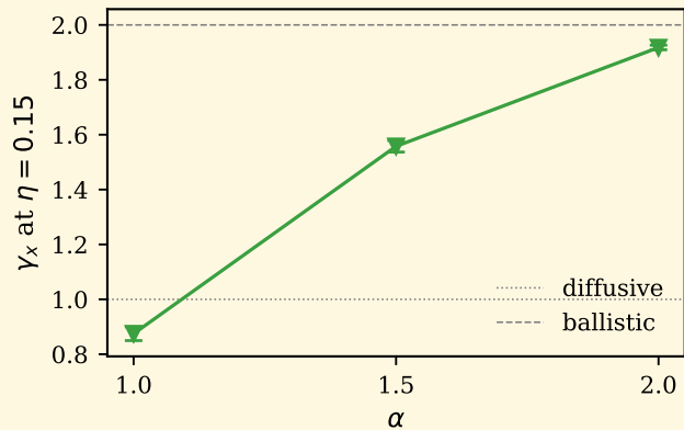
(c) spatial MSD exponent
