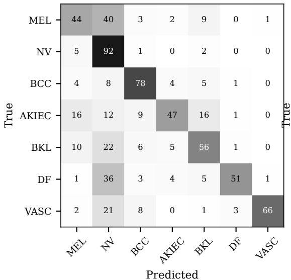
Federated ( \alpha=0.5 )
