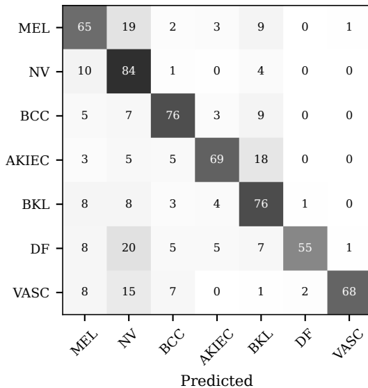
Centralized
