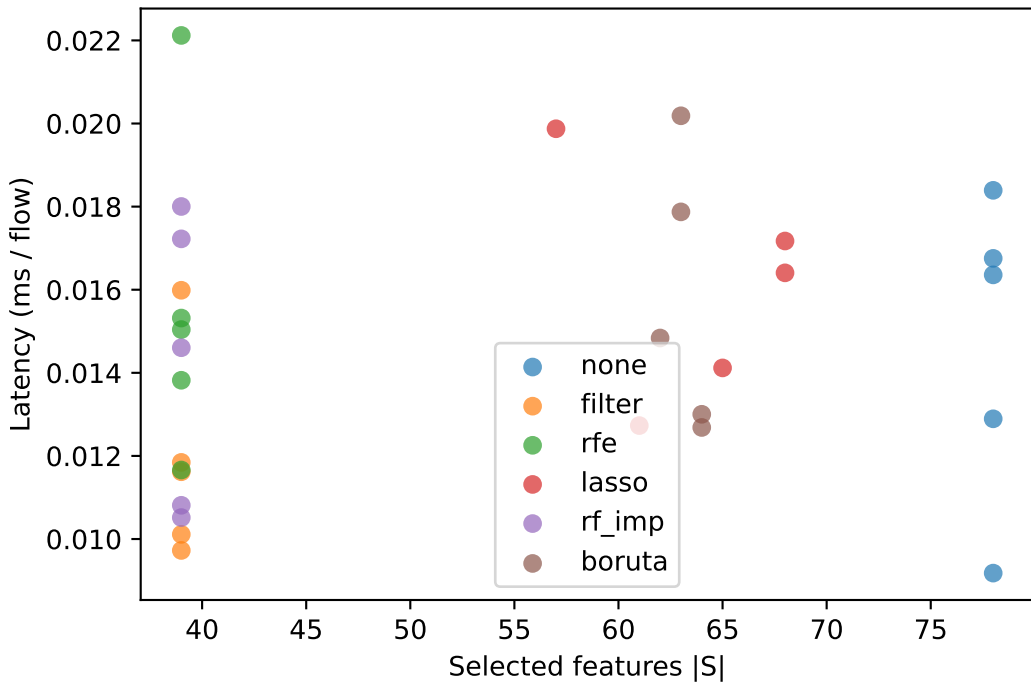
Inference latency vs subset size
