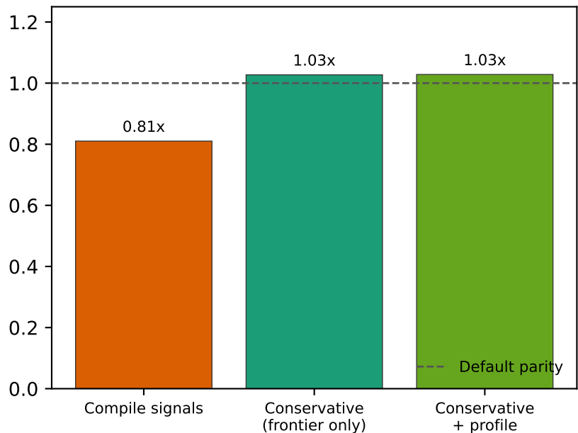
Reduction split removed: conservative selector recovers parity
