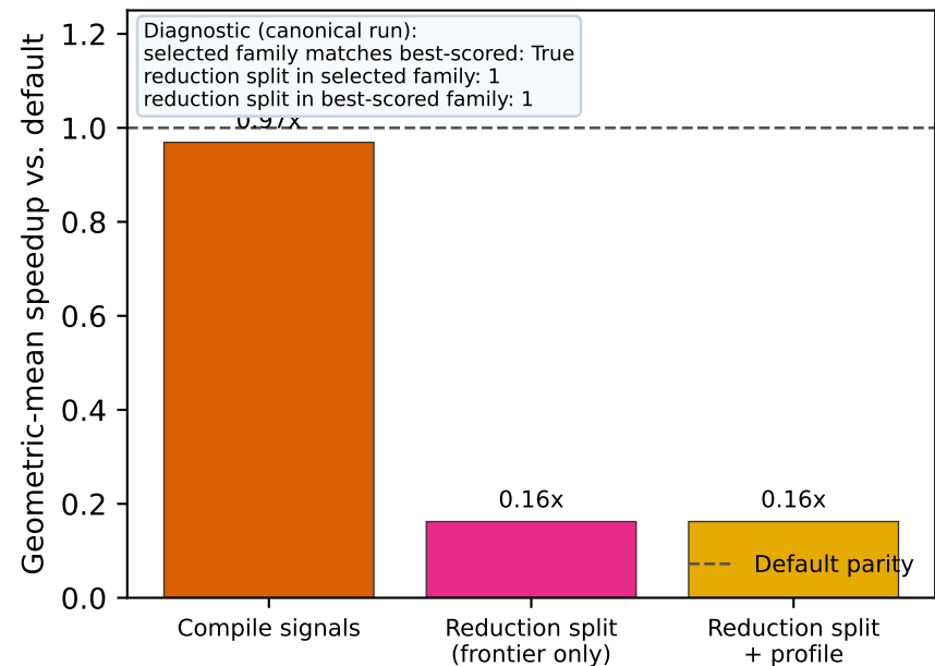
Enlarged search space: reduction-split variants collapse
