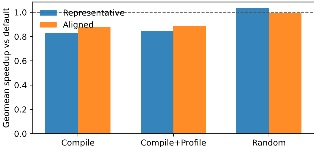
Aligned workloads flatter selector quality
