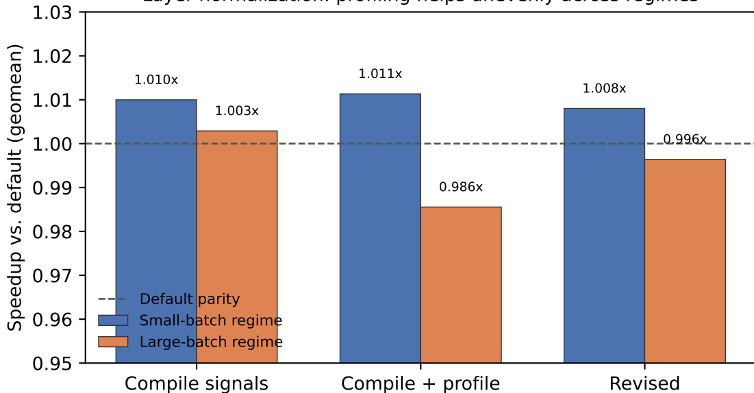
Layer normalization: profiling helps unevenly across regimes
