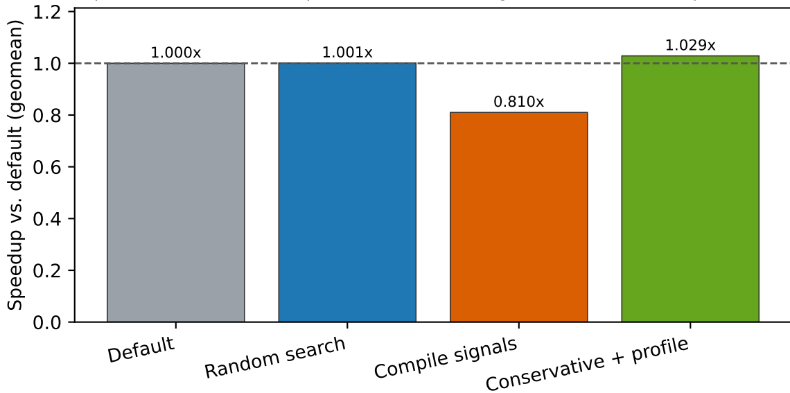
Representative matrix multiplication, matched budget (12 benchmarks, 4 profile runs)
