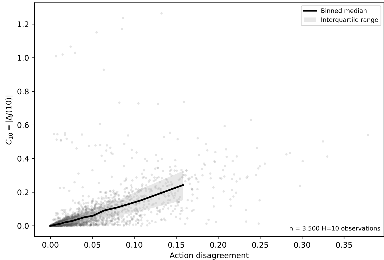
Counterfactual consequence vs. action disagreement
