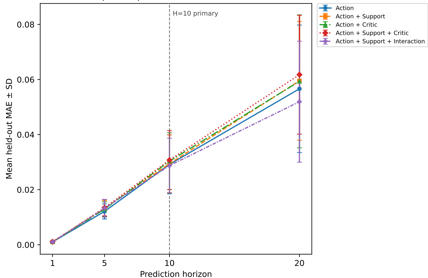
Held-out consequence prediction across downstream horizons
