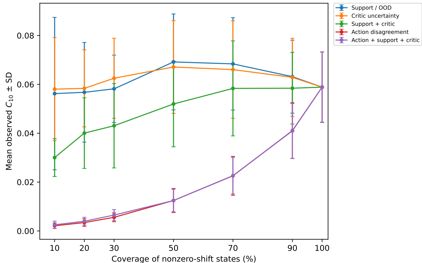
Reliability-score risk-coverage ( \sigma > 0 )
