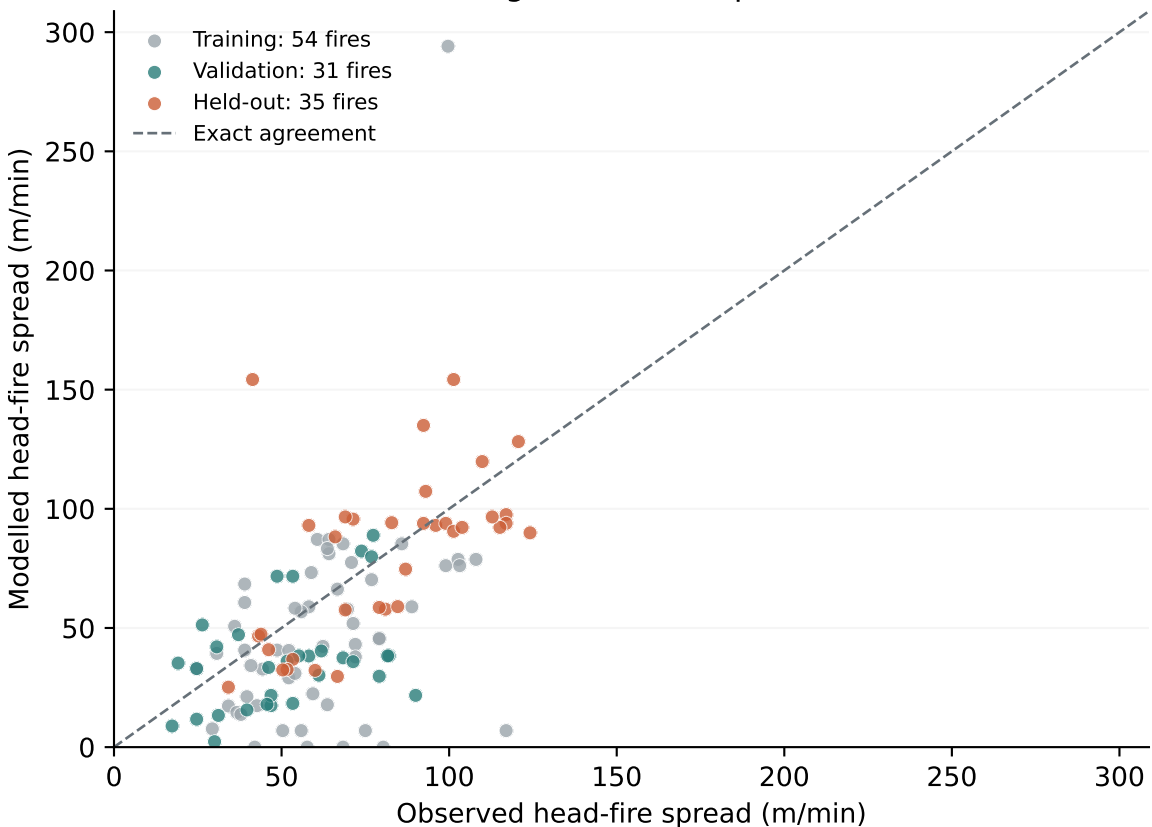
Historical grass-fire component test
