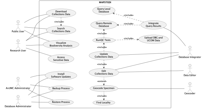
Figure 4: MAPSTEDI subsystem use case diagram used as the real-world evaluation input.
