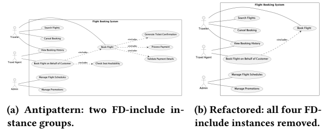
Figure 2: Flight Booking System: antipattern and refactored diagrams.
