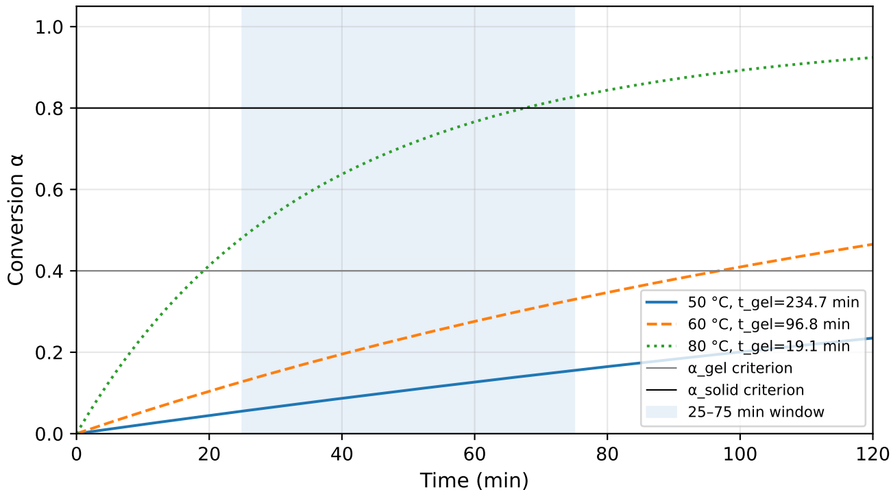
Phenomenological conversion vs time (inhibitor index = 0.6)
