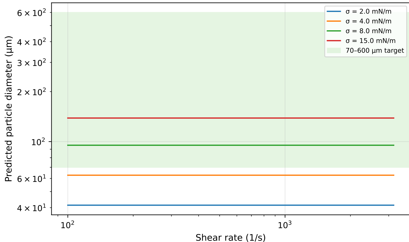
Hinze/Grace characteristic diameter vs shear and IFT
