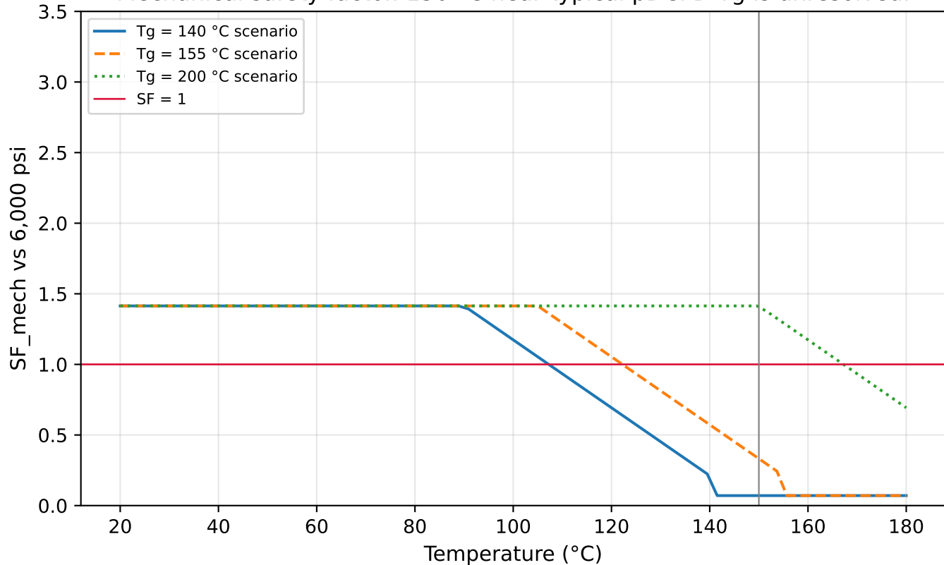
Mechanical safety factor. 150 °C near typical pDCPD Tg is unresolved.
