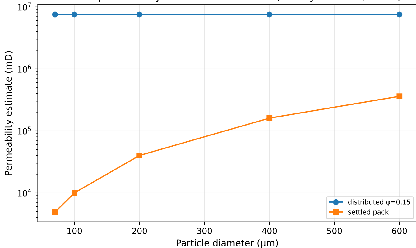
Residual permeability: distributed vs settled (Kozeny-Carman / dilute)
