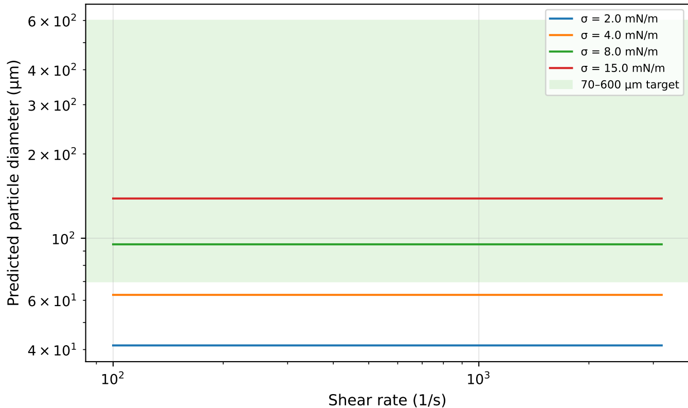
Hinze/Grace characteristic diameter vs shear and IFT (order-of-magnitude)
