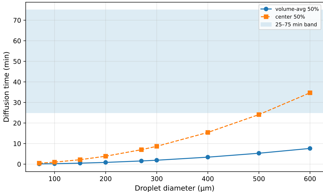
Diameter vs activator diffusion time (Lee ambient D)
