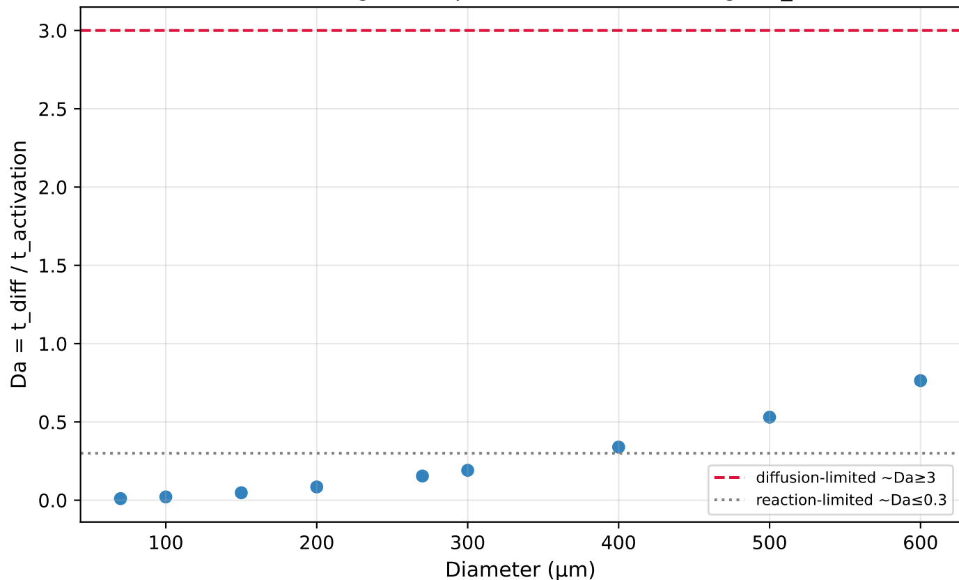
Damköhler regime map (Lee ambient D, analogue t_{act} )
