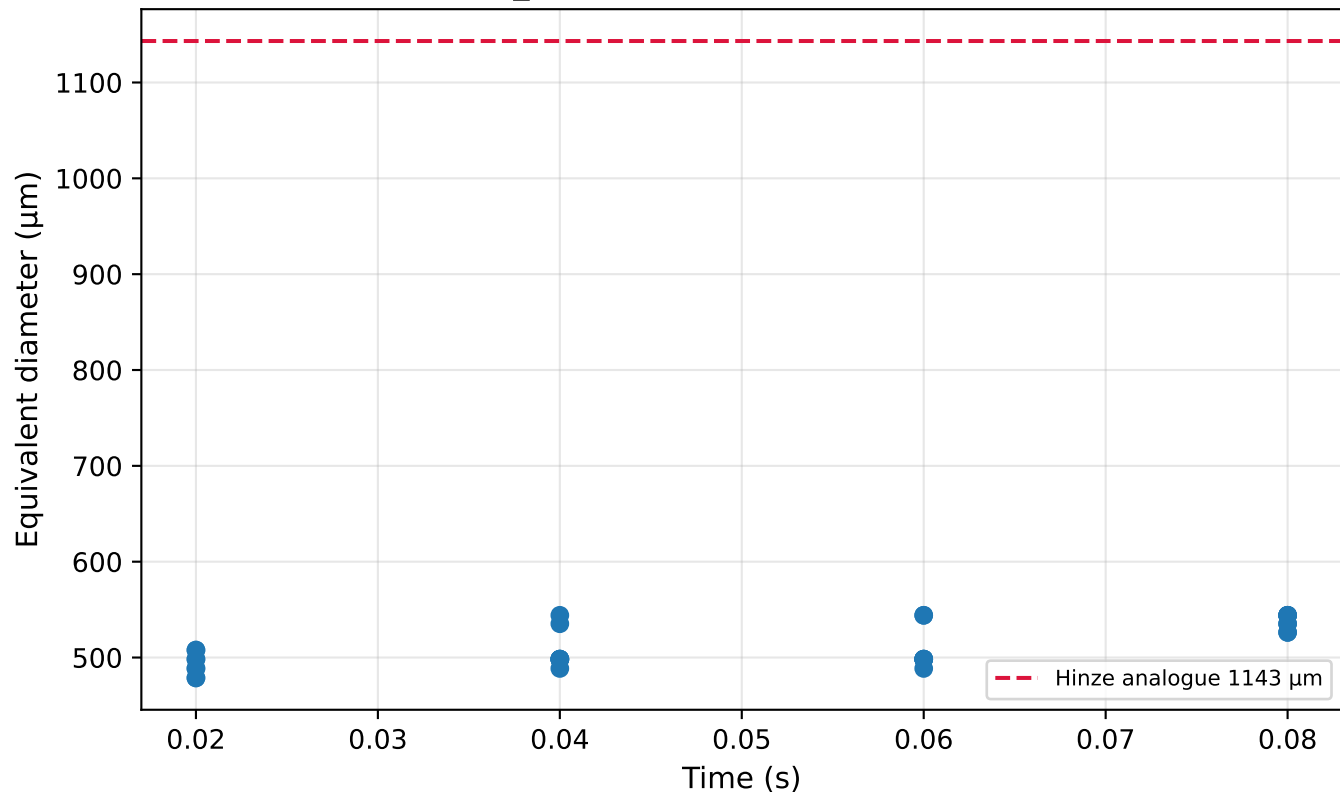
CFD d_eq vs Hinze/Grace-scale estimate
