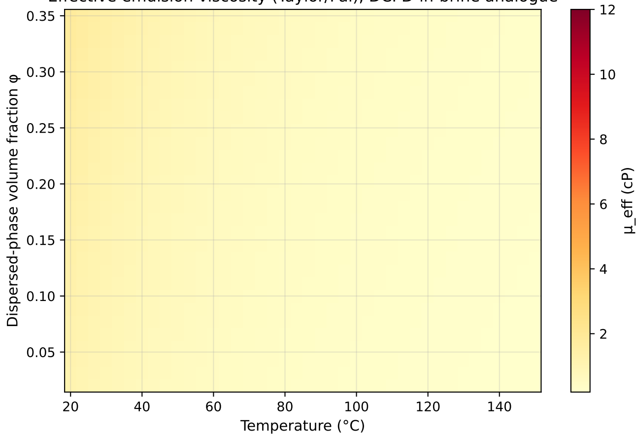
Effective emulsion viscosity (Taylor/Pal), DCPD-in-brine analogue
