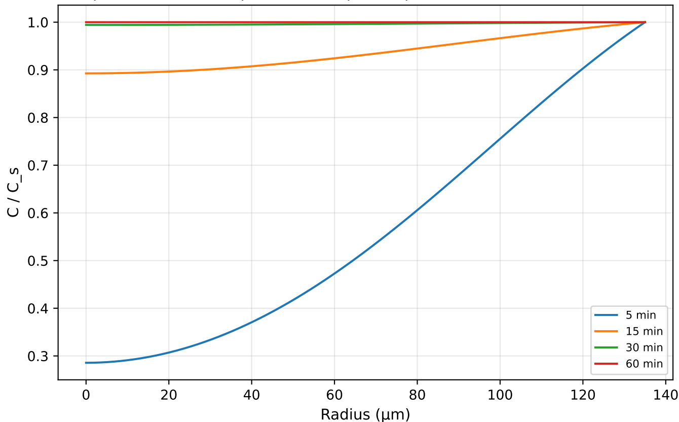
Spherical activator profiles, 270 \mu\text{m} drop, Lee ambient D (not 150 ^{\circ}\text{C} )
