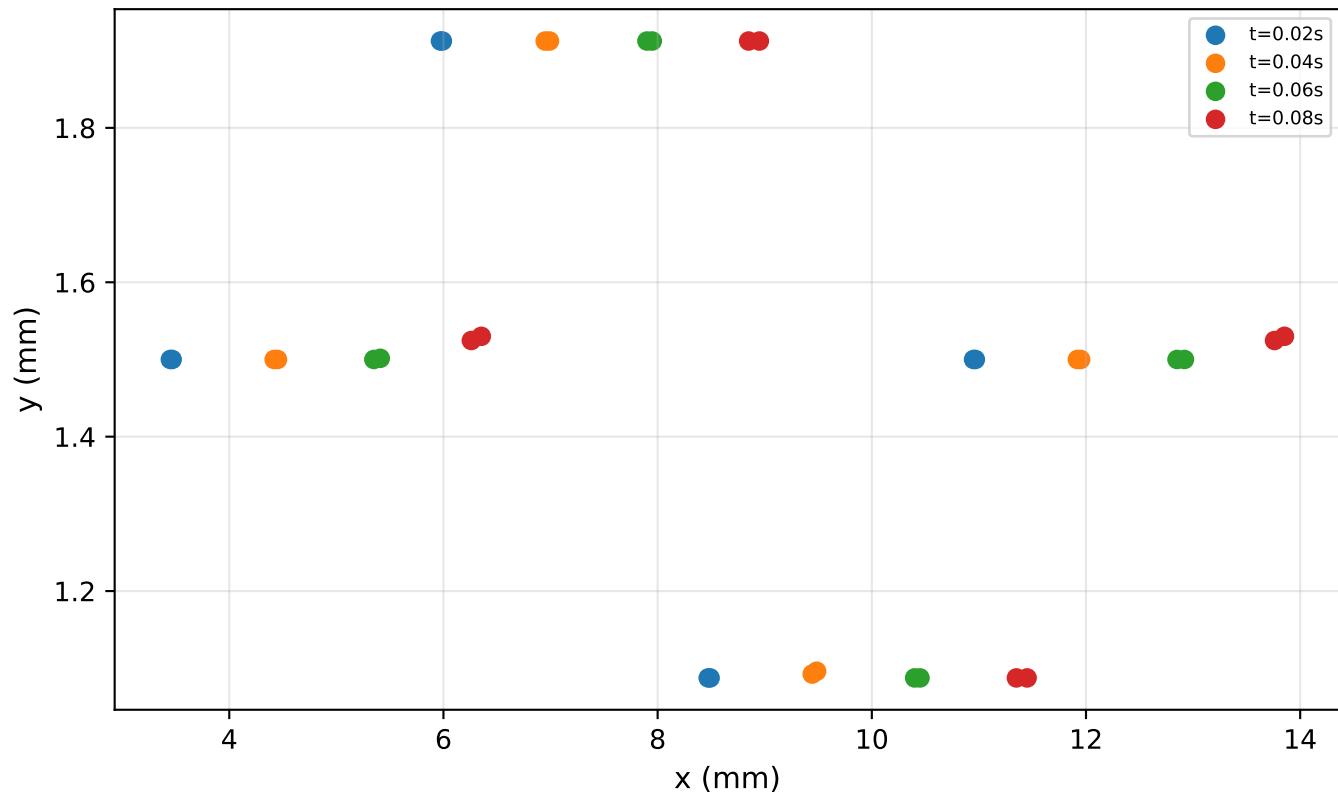
CFD droplet centroids (model prediction)
