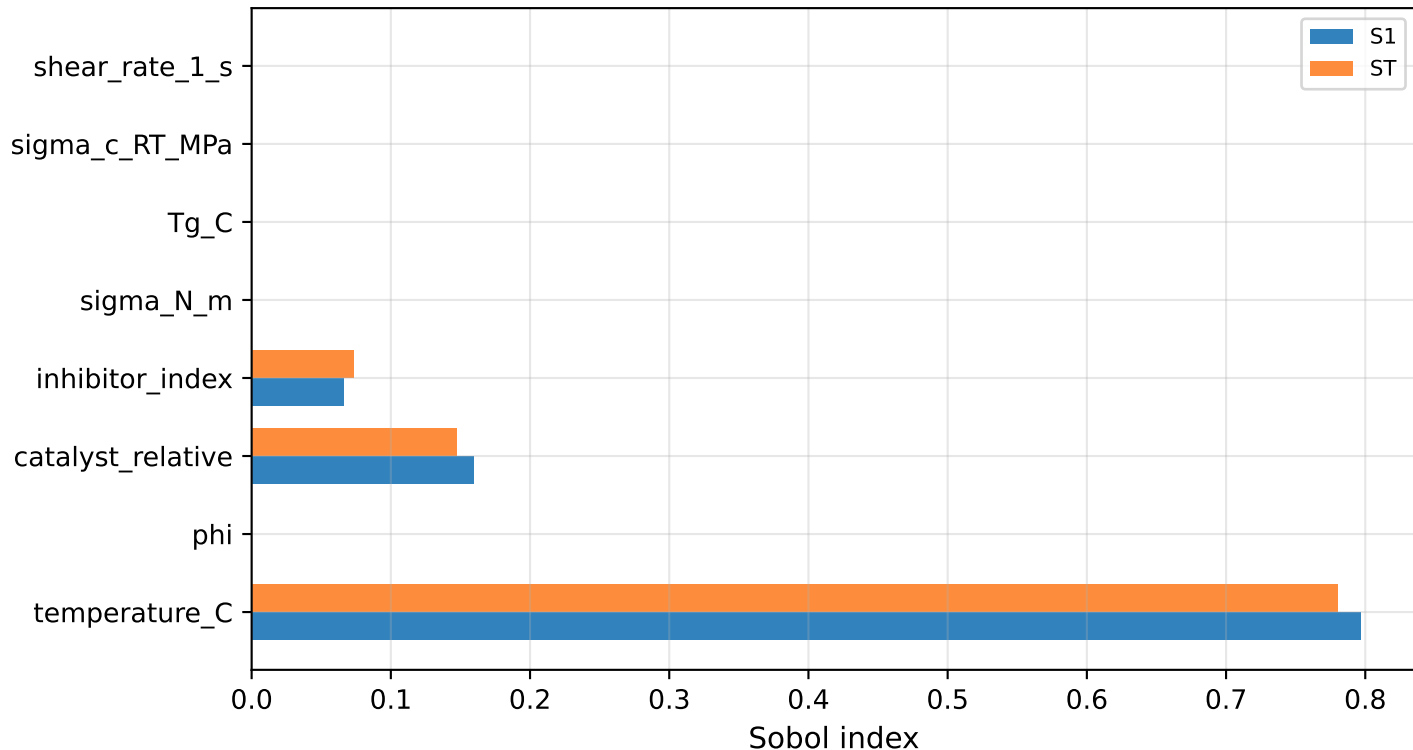
Global sensitivity of \log_{10}(t_{\text{transform}}) (40–90 °C envelope)
