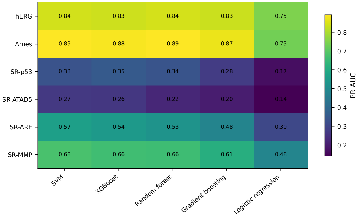
Scaffold-aware test performance: PR-AUC
