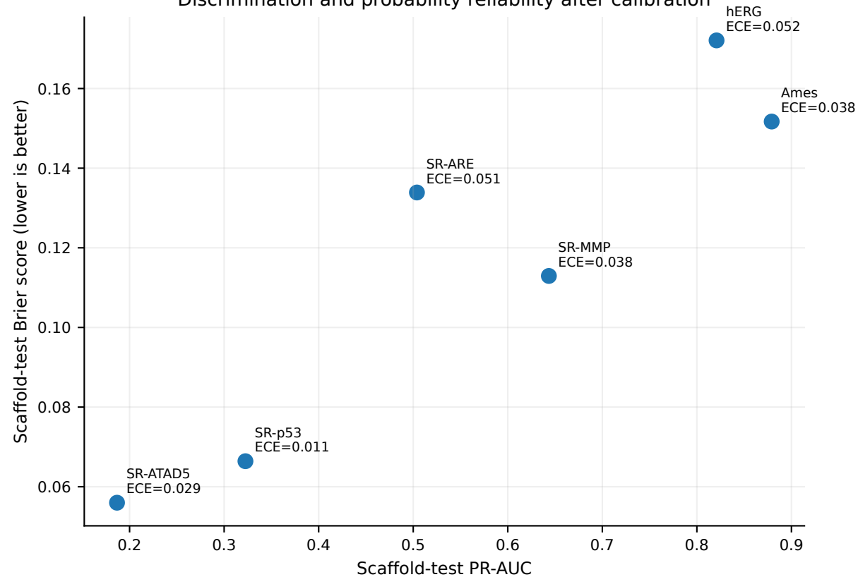
Discrimination and probability reliability after calibration
