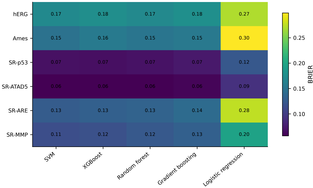
Scaffold-aware test reliability: Brier score
