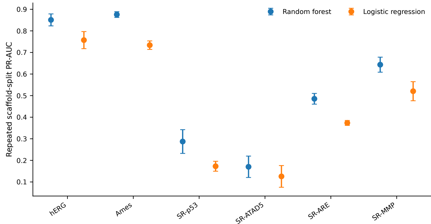
Five-run scaffold-split stability (mean and 95% CI)
