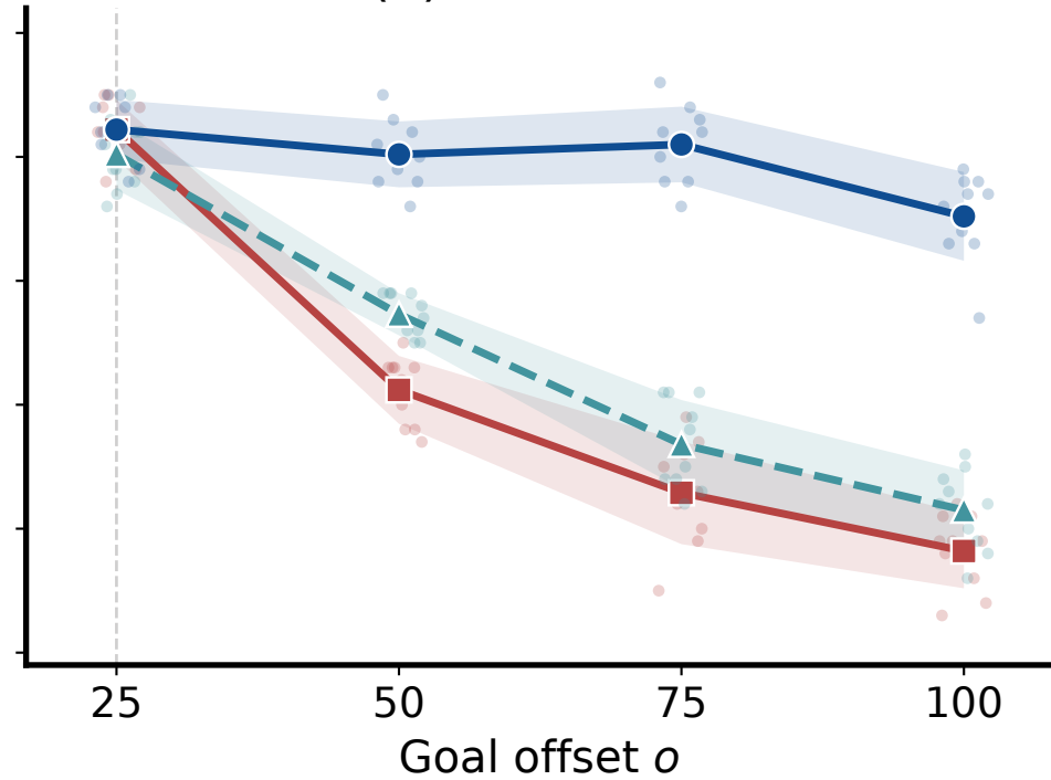
(b) TwoRoom
