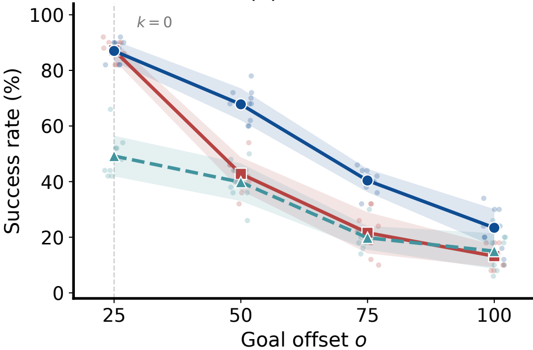
(a) PushT
