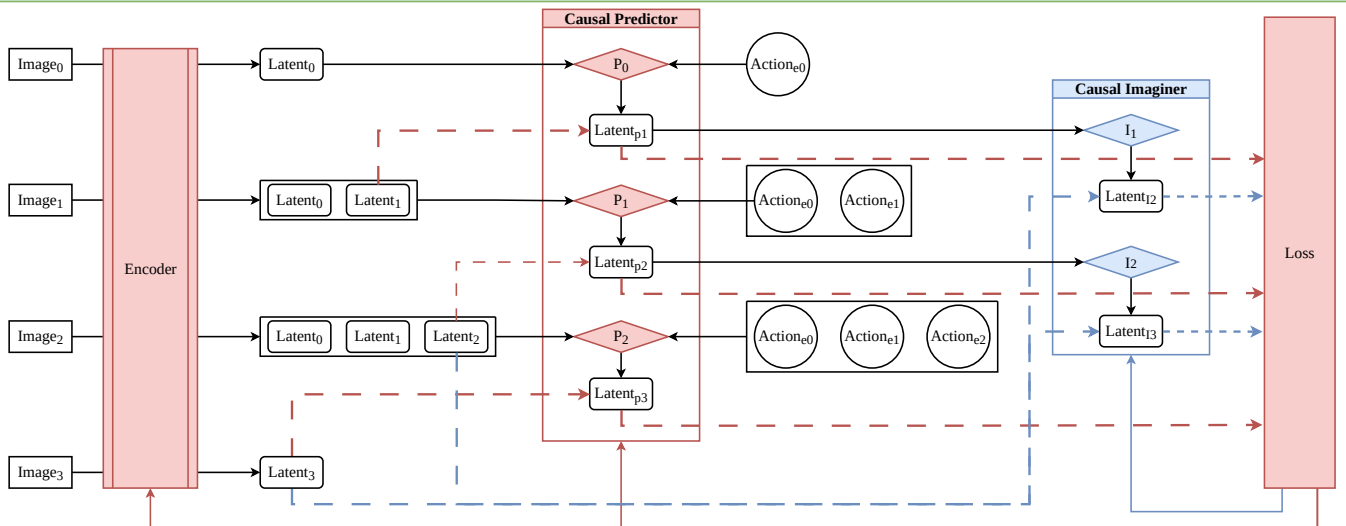
Auto-Forward LeWM Training Pipeline
