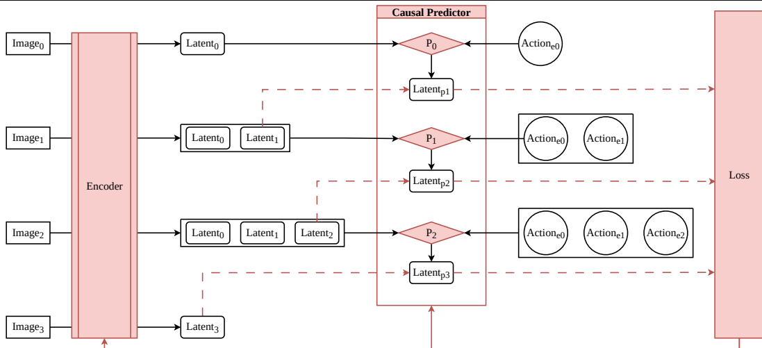
Auto-Forward LeWM Training Pipeline
