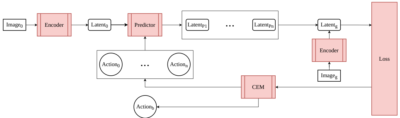
HAS Evaluation Pipeline
