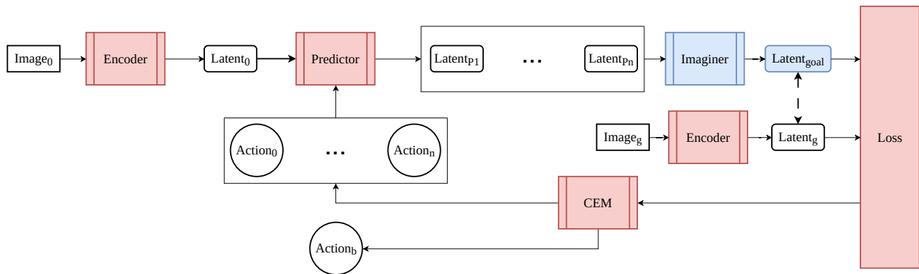
Auto-Forward LeWM Eval Pipeline
