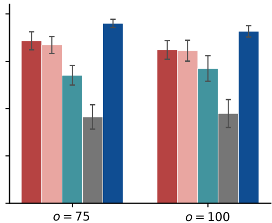
Reacher
