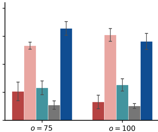
TwoRoom
