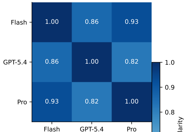
ALFWORLD - Tower
