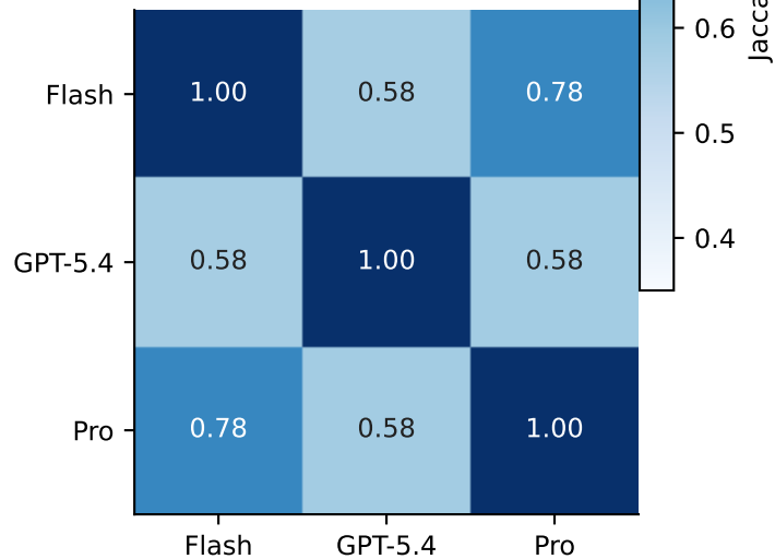
WEBSHOP - Tower
