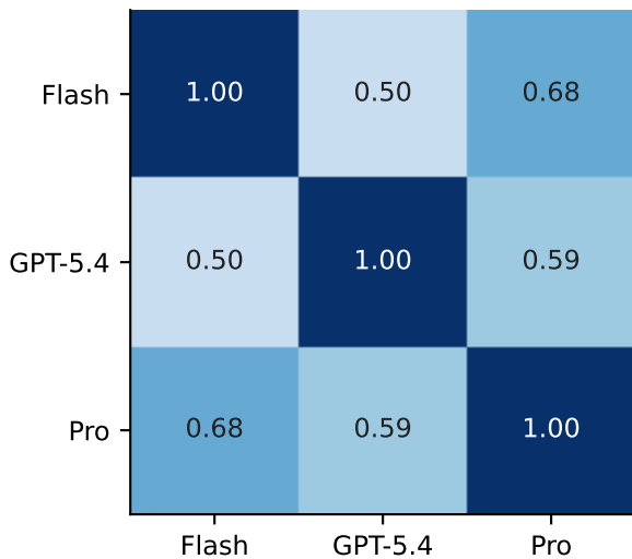
WEBSHOP - No-Skill
